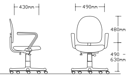
Chrome base and castors
