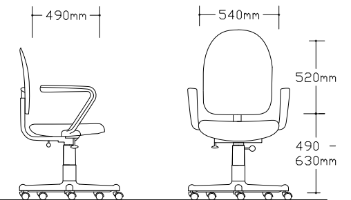
Chrome base and castors with adj. arms
